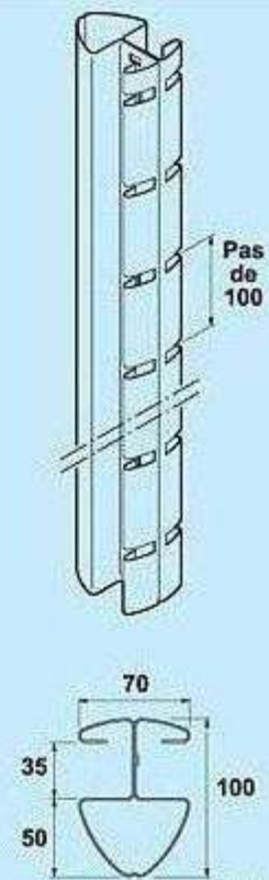
stub Axis 100/50 mm
