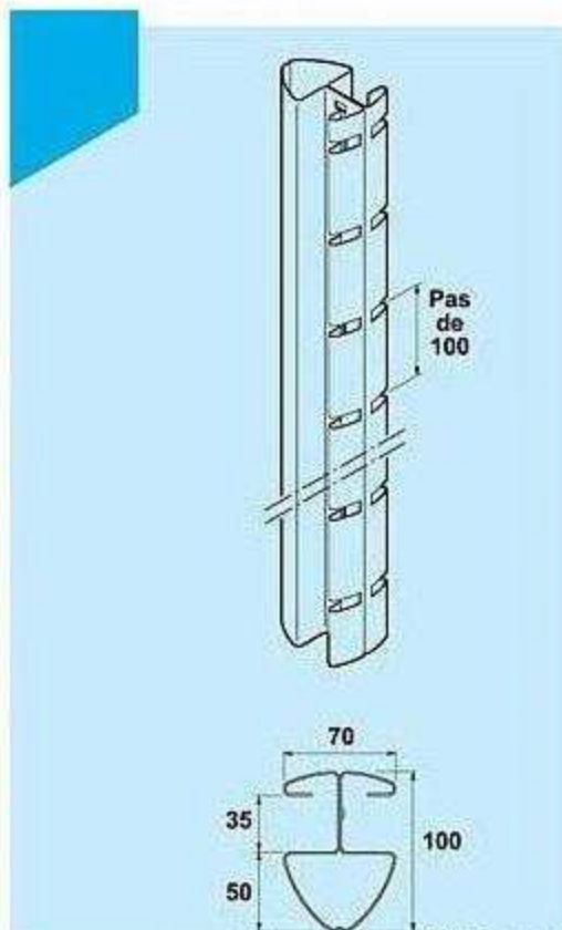
stub Axis 100/50 mm
